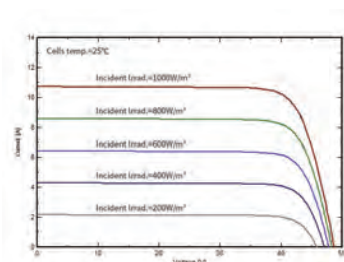
I-V Curve at different irradiation (SPP415DH7H)
